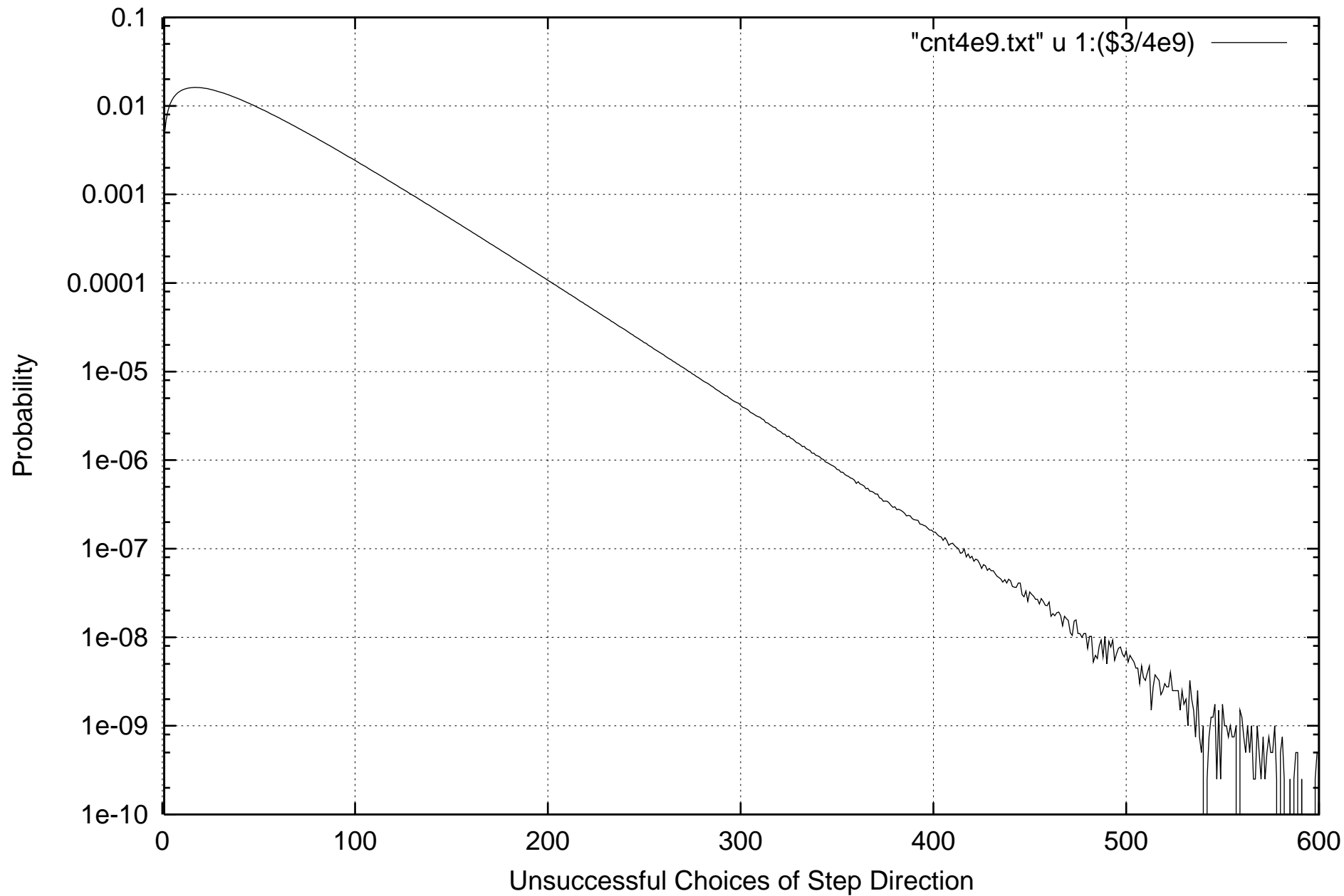
Self-Trapping Random Walk on 2-D Lattice ( 4 \cdot 10^9 Walks)
