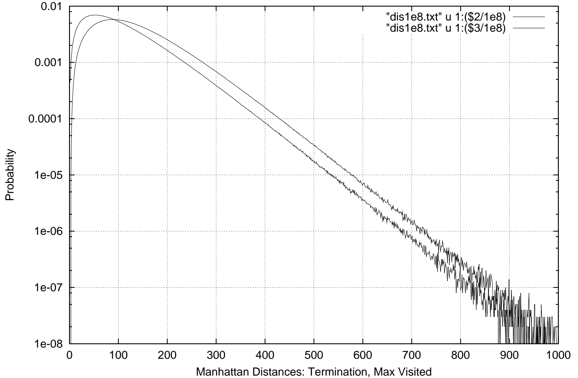
Self-Trapping Random Walk on 3-D Lattice ( 10^8 Walks)
