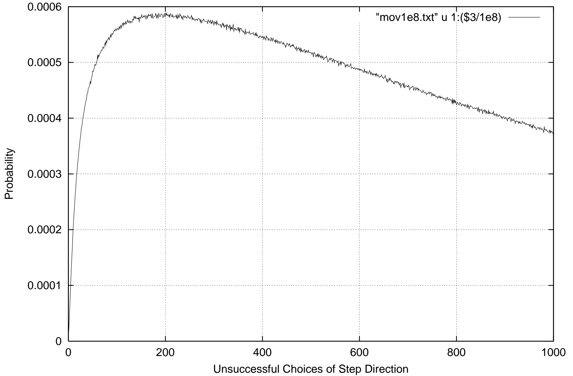
Self-Trapping Random Walk on 3-D Lattice (10 8 Walks)
