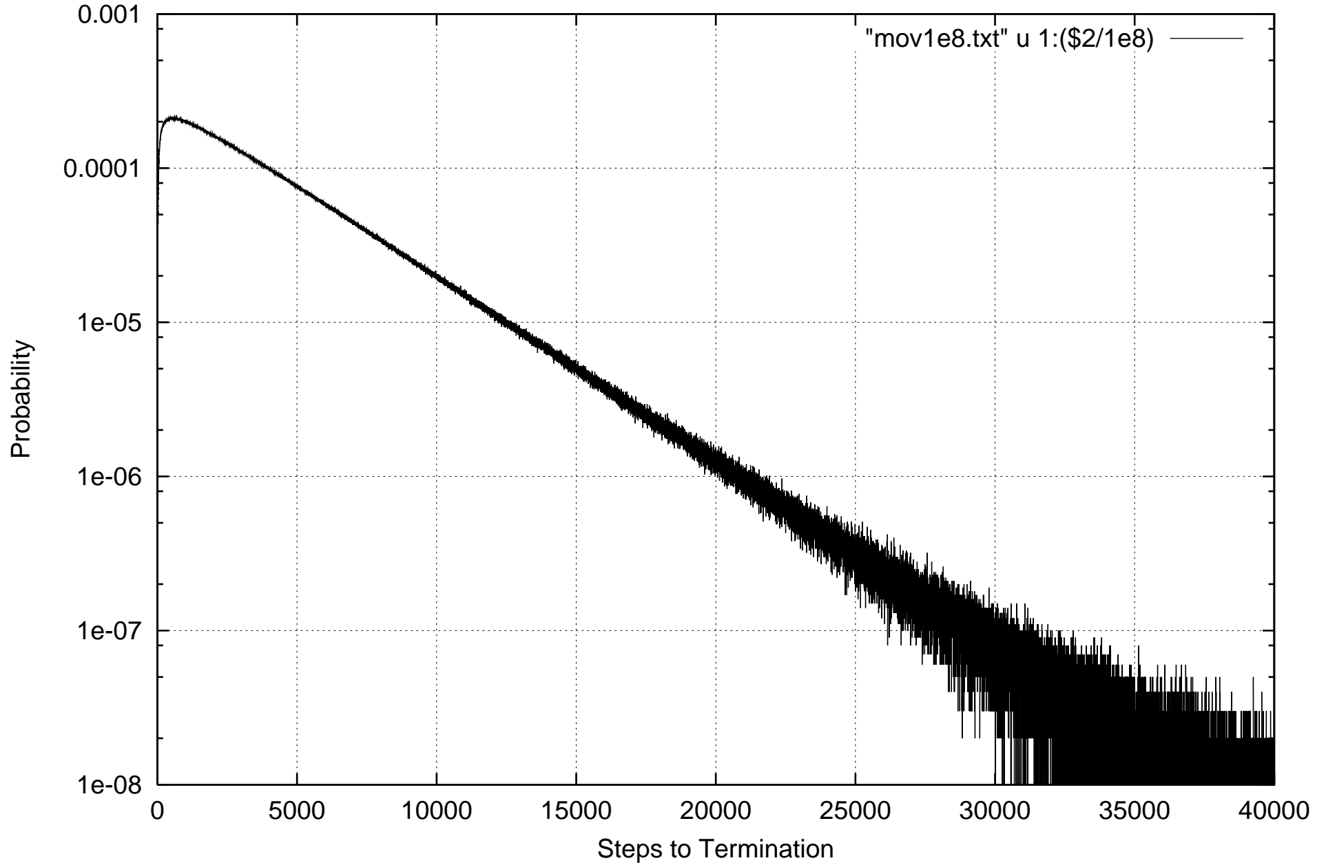
Self-Trapping Random Walk on 3-D Lattice (10 8 Walks)
